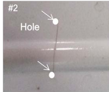
#2 Drill a hole about 1/8 of an inch in size at either side of the crack near its end points to prevent the crack from becoming bigger
